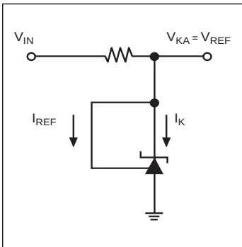
Figure 2. Test Circuit for V_{KA} = V_{REF}
