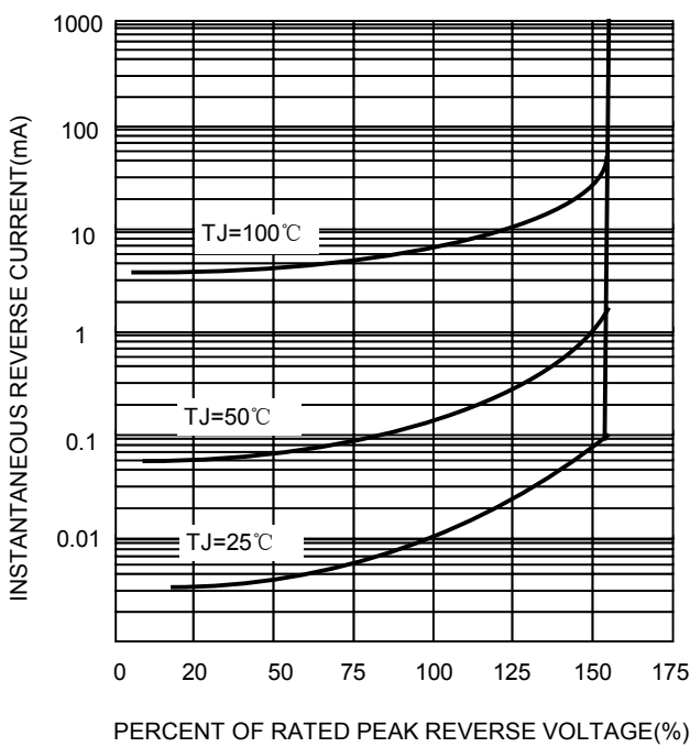
FIG.3-TYPICAL REVERSE CHARACTERISTICS
