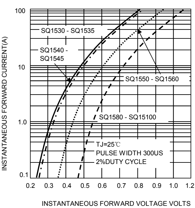
FIG.4-TYPICAL FORWARD CHARACTERISTICS
