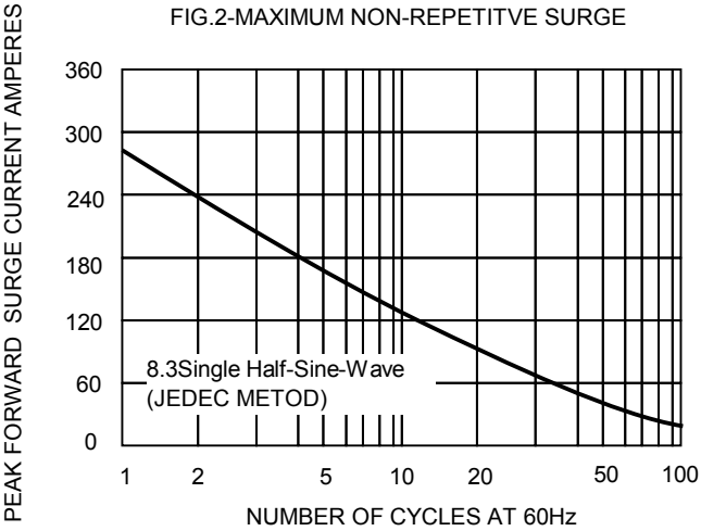
FIG.2-MAXIMUM NON-REPETITIVE SURGE
