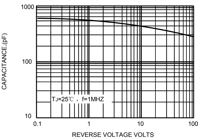
FIG.5-TYPICAL JUNCTION CAPACITANCE
