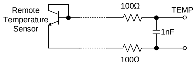
Figure 18. Filter Between Remote Sensor and SQ24905C
