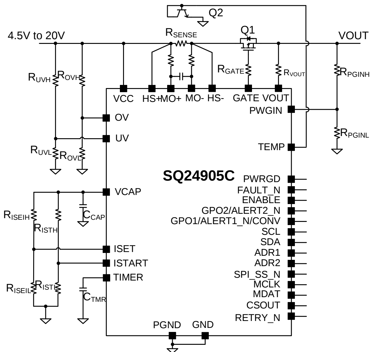
Figure 1. Schematic Diagram
