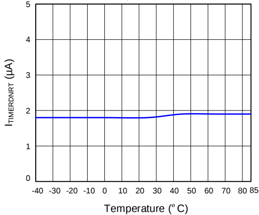
TIMER Pull-Down Current Retry ( I_{\text{TIMERDNRRT}} ) vs. Temperature
