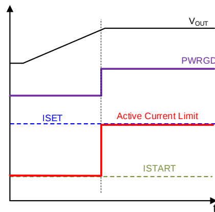
Figure 9. Interaction of ISTART and ISET Current Limits
