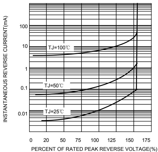
FIG.3-TYPICAL REVERSE CHARACTERISTICS
