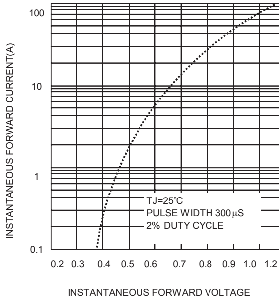
FIG.4-TYPICAL FORWARD CHARACTERISTICS
