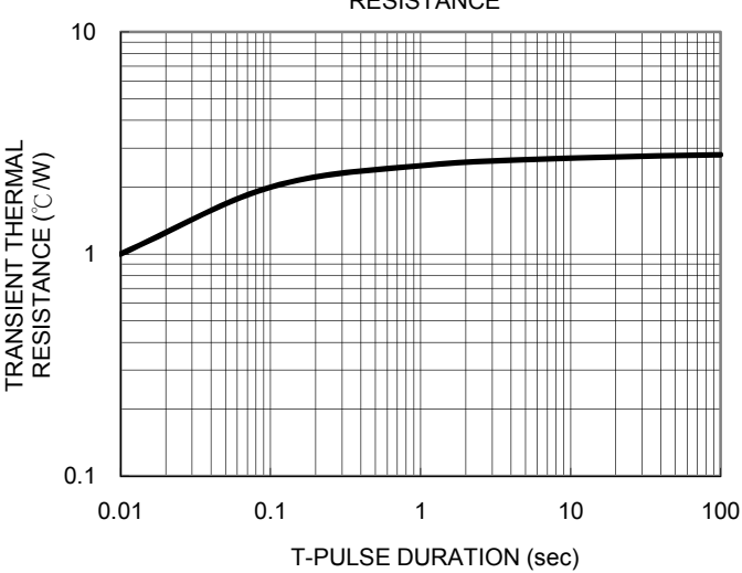
FIG. 6 TYPICAL TRANSIENT THERMAL RESISTANCE
