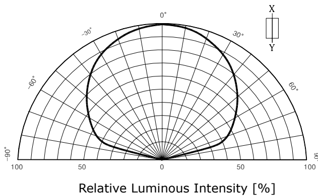
Fig. 5-1 Radiation Diagram
