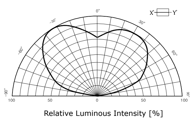
Fig. 5-2 Radiation Diagram
