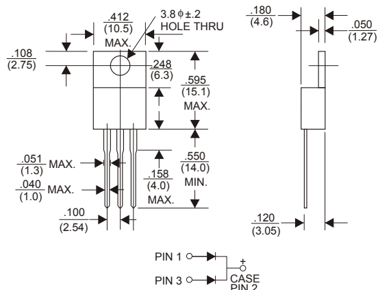
TO-220
