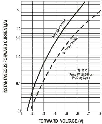
FIG.2-TYPICAL FORWARD CHARACTERISTICS
