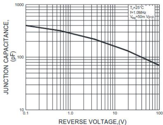
FIG.5-TYPICAL JUNCTION CAPACITANCE
