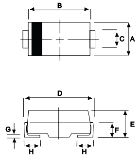
DO-214AA(SMB)
