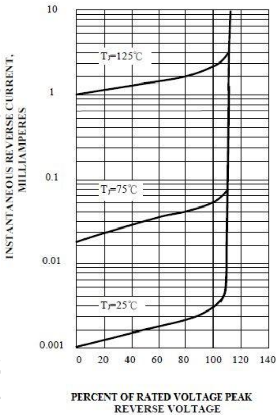
FIG. 3 - TYPICAL REVERSE
