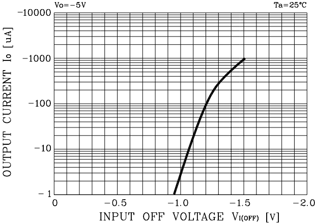
Fig. 2 I_o - V_{I(OFF)}
