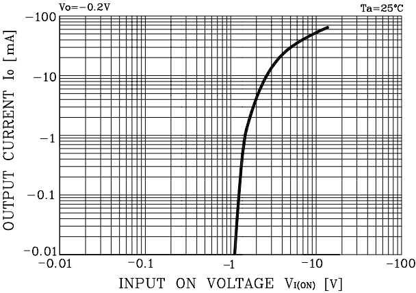
Fig. 1 I_o - V_{I(ON)}
