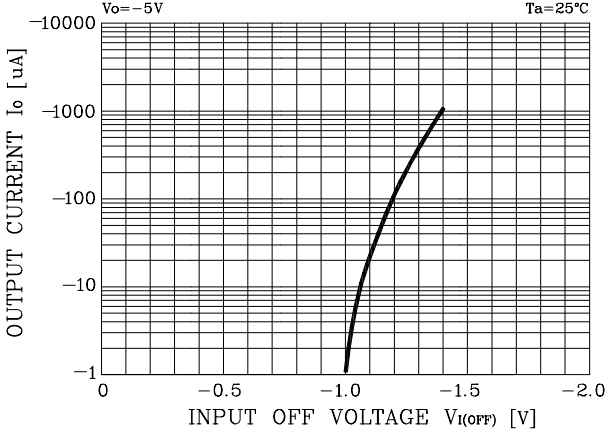
Fig. 2 I_o - V_{I(OFF)}
