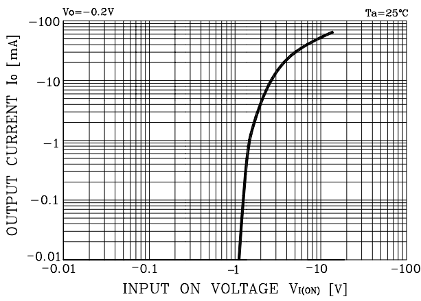
Fig. 1 I_o - V_{I(ON)}
