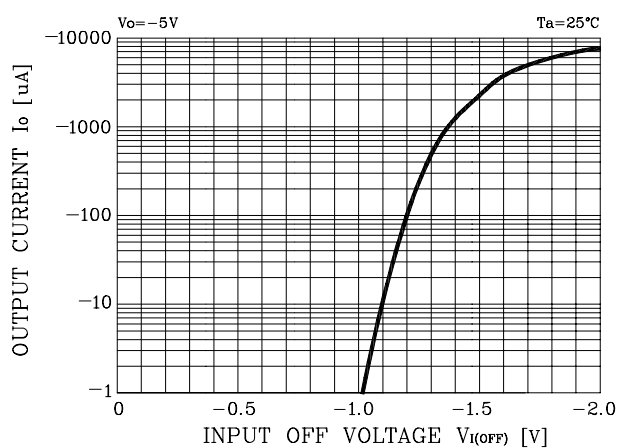
Fig. 2 I_O - V_{I(OFF)}
