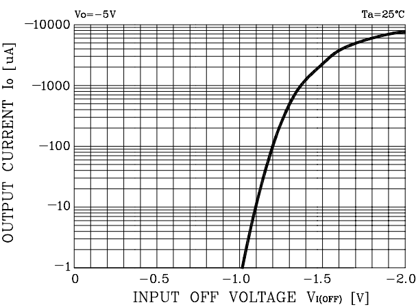
Fig. 2 I_o - V_{I(OFF)}
