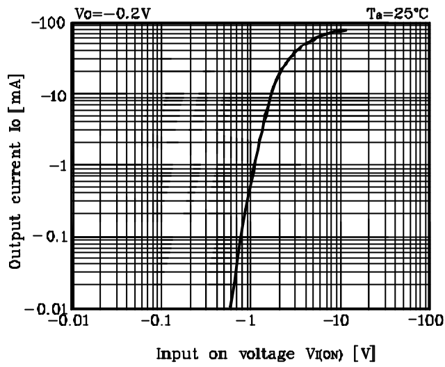
Fig. 1 I_O - V_{I(ON)}
