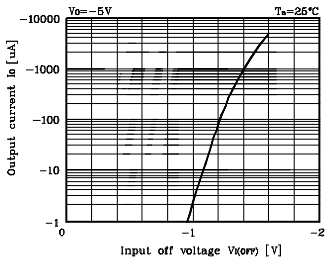
Fig. 2 I_O - V_{I(OFF)}
