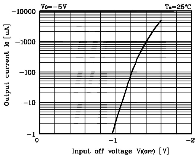
Fig. 2 I_O - V_{I(OFF)}
