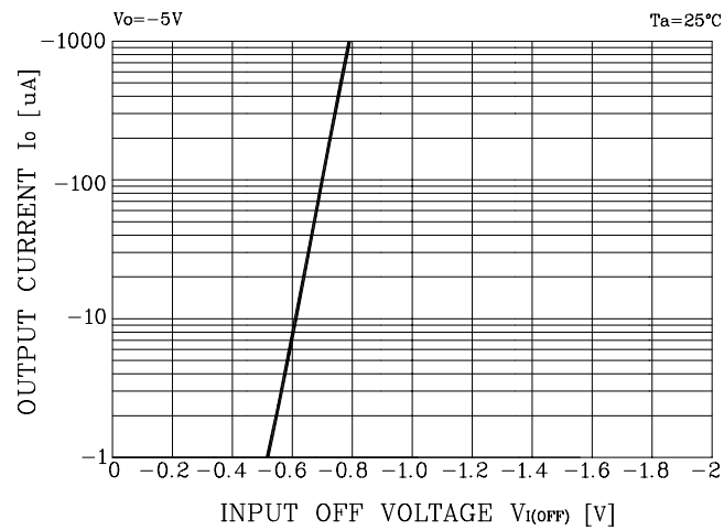
Fig. 2 I_o - V_{I(OFF)}
