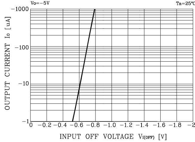
Fig. 2 I_o - V_{I(OFF)}
