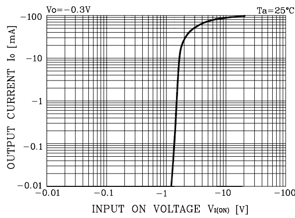
Fig. 1 I_O - V_{I(ON)}
