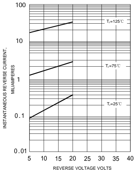
FIG.2-TYPICAL REVERSE CHARACTERISTICS
