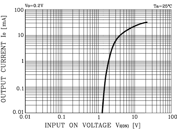
Fig. 1 I_O - V_{I(ON)}
