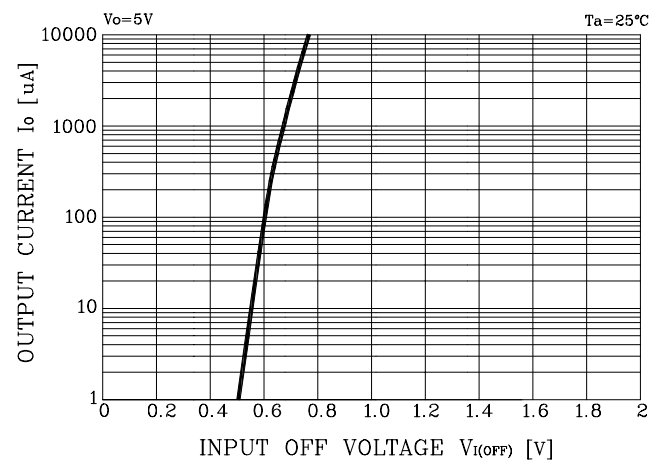
Fig. 2 I_O - V_{I(OFF)}
