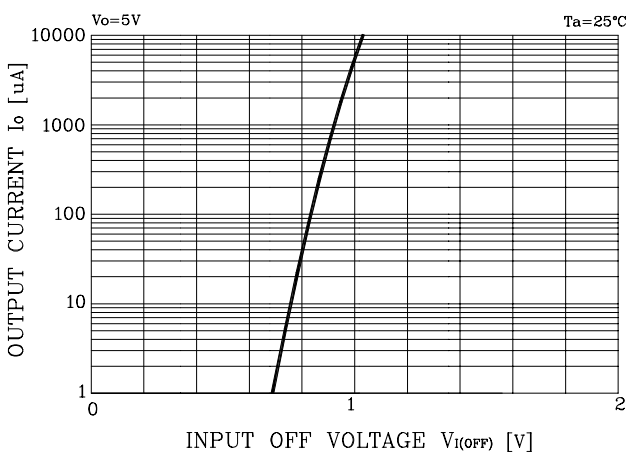
Fig. 2 I_O - V_{I(OFF)}
