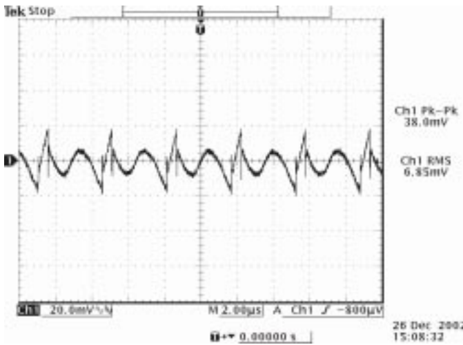
Ripple and noise at full load and 8Vdc input, 1.0Vdc output and T_a=25^\circ\text{C}
