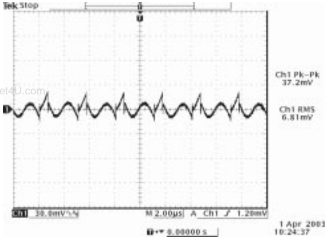
Ripple and noise at full load and 8Vdc input, 1.5Vdc output and T_a=25^\circ\text{C}
