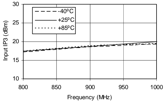
Input IP3 vs Temperature
