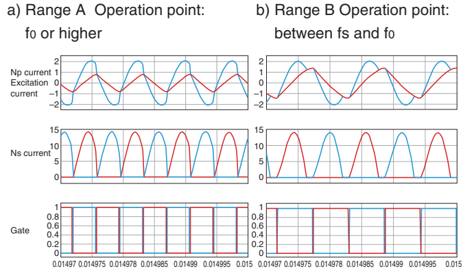
Figure 5 Operation waveform in each mode
