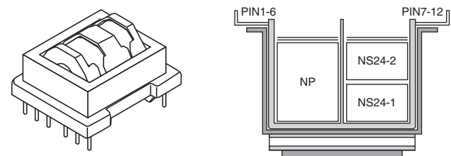
Figure 9 Split winding structure
