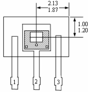
Sensor Location
