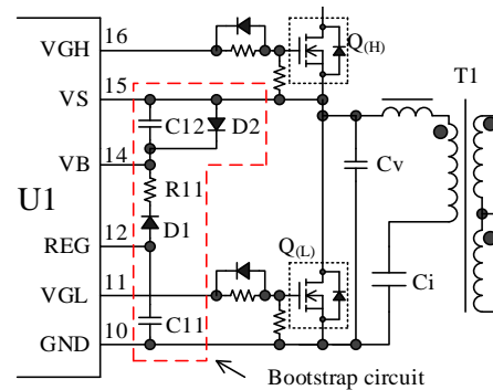
Figure 8-16. Bootstrap Circuit
