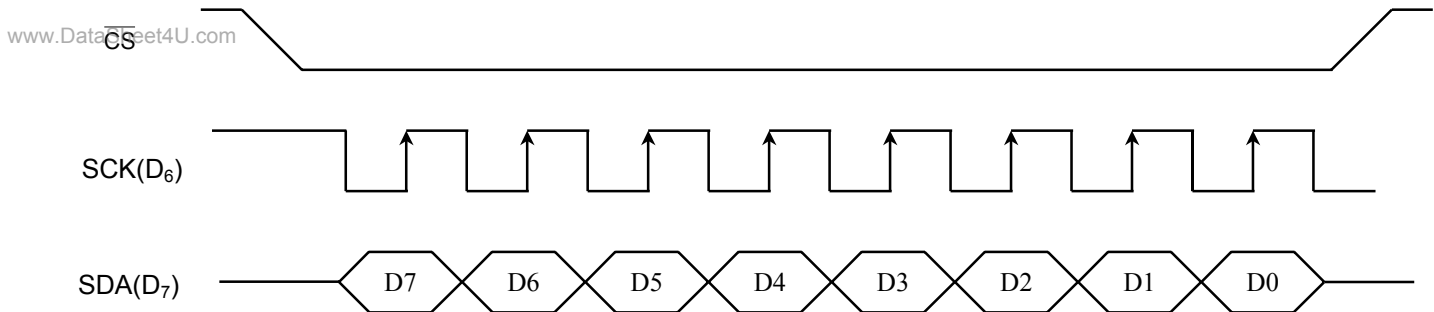
Figure 21 - Serial Timing Characteristics (PS0 = L, PS1 = L)
