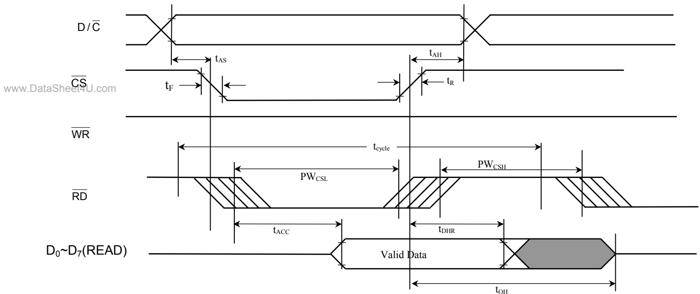
Figure 20 – Parallel 8080-series Interface Timing Characteristics (PS0 = H, PS1 = L)
