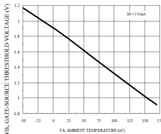
Figure 9. Threshold Voltage
