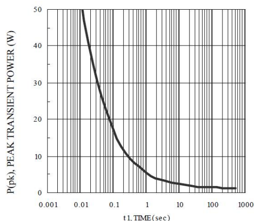
Figure 10. Single Pulse Power
