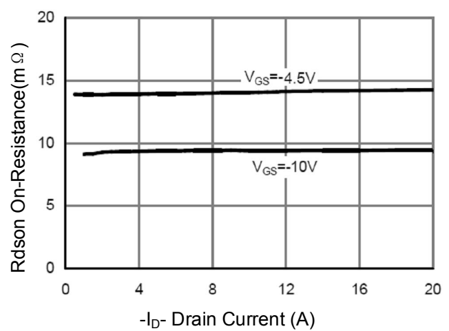
Figure 6 Drain-Source On-Resistance
