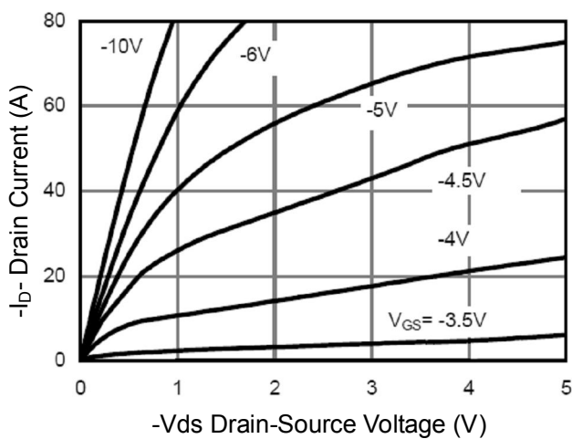
Figure 5 Output CHARACTERISTICS
