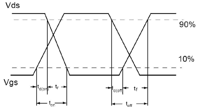
Figure 2: Switching Waveform
