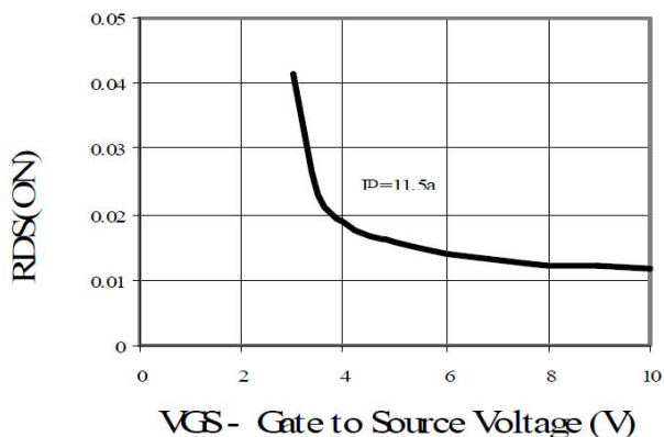
Figure 4. On-Resistance with Gate to Source Voltage
