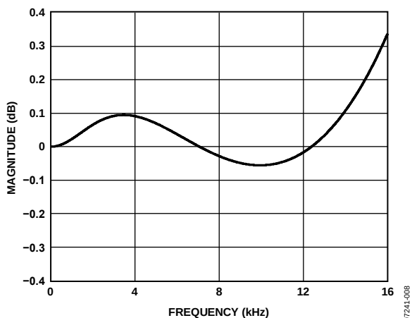
Figure 12. De-Emphasis Error, Audio Sampling Rate = 32 kHz
