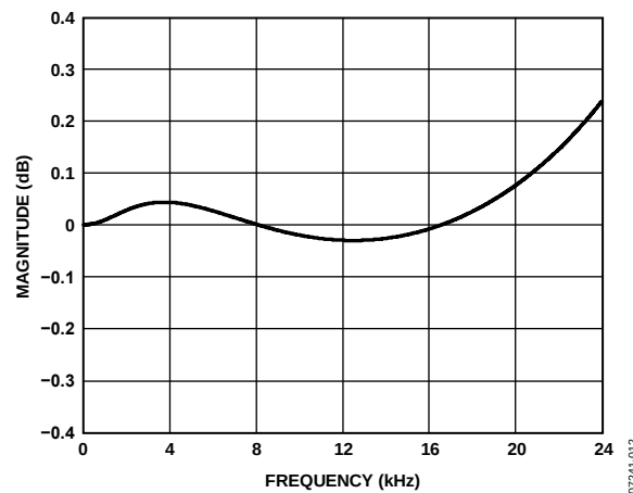
Figure 16. De-Emphasis Error, Audio Sampling Rate = 48 kHz
