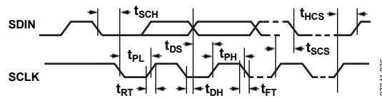
Figure 2. I 2 C Timing
