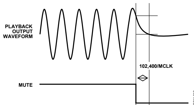
Figure 17. Enabling of MUTE
