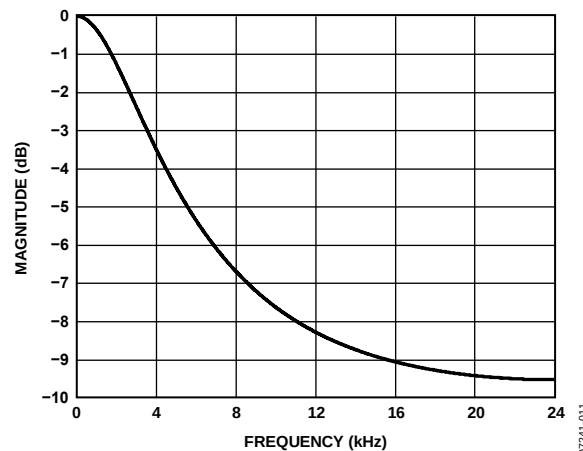
Figure 15. De-Emphasis Frequency Response, Audio Sampling Rate = 48 kHz
