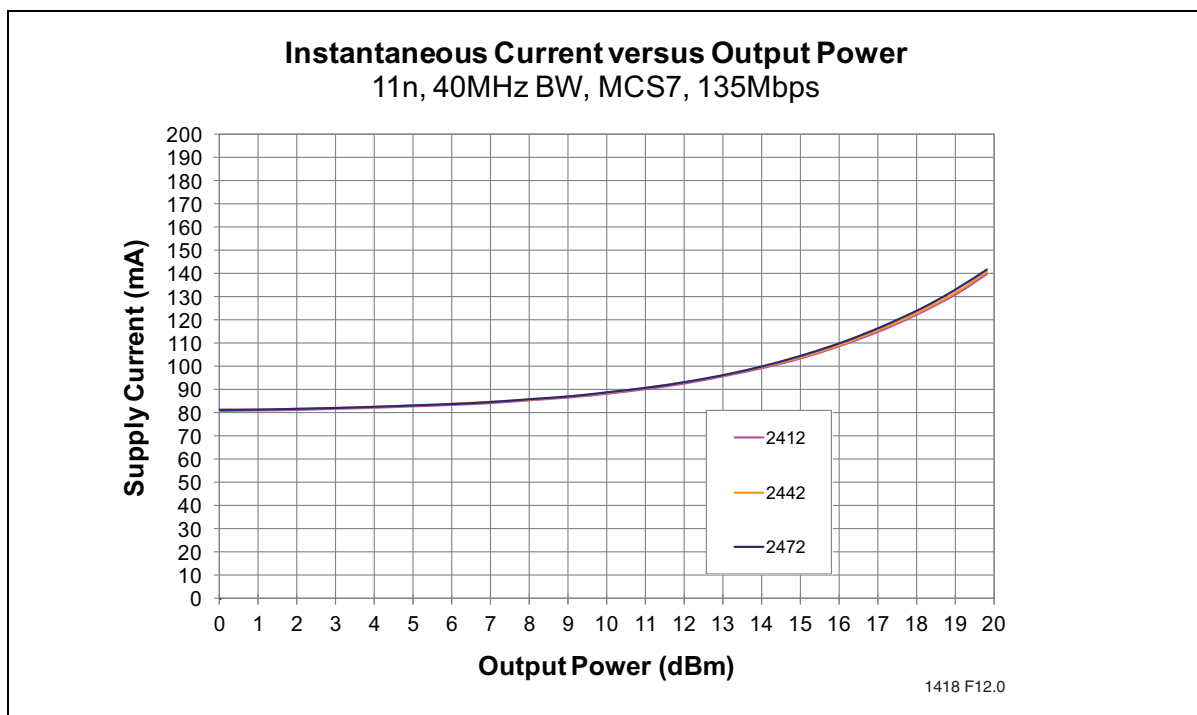
Figure 9: Total Current Consumption for 11n and 256 QAM Operations
