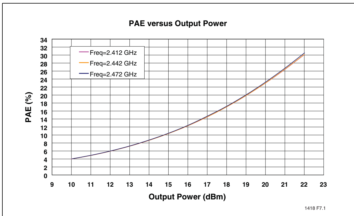
Figure 10: PAE versus Output Power
