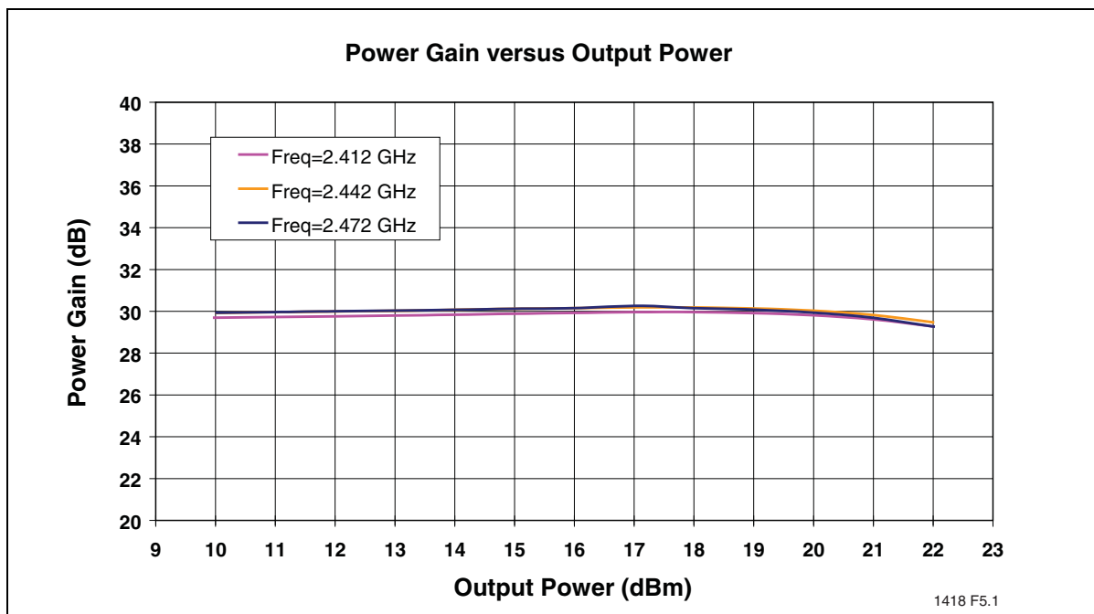
Figure 7: Power Gain versus Output Power
