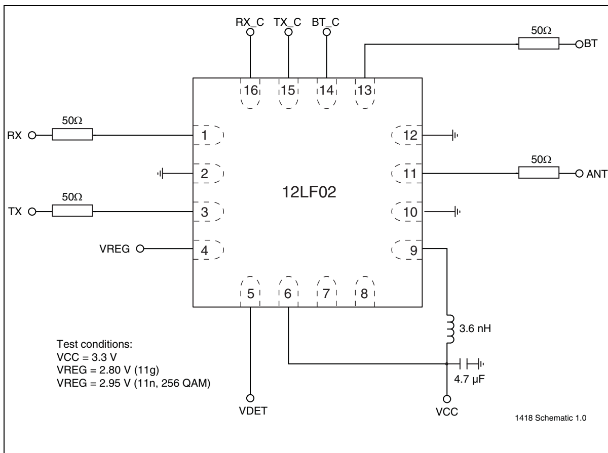
Figure 12: Typical Schematic for High-Efficiency 802.11b/g/n Applications
