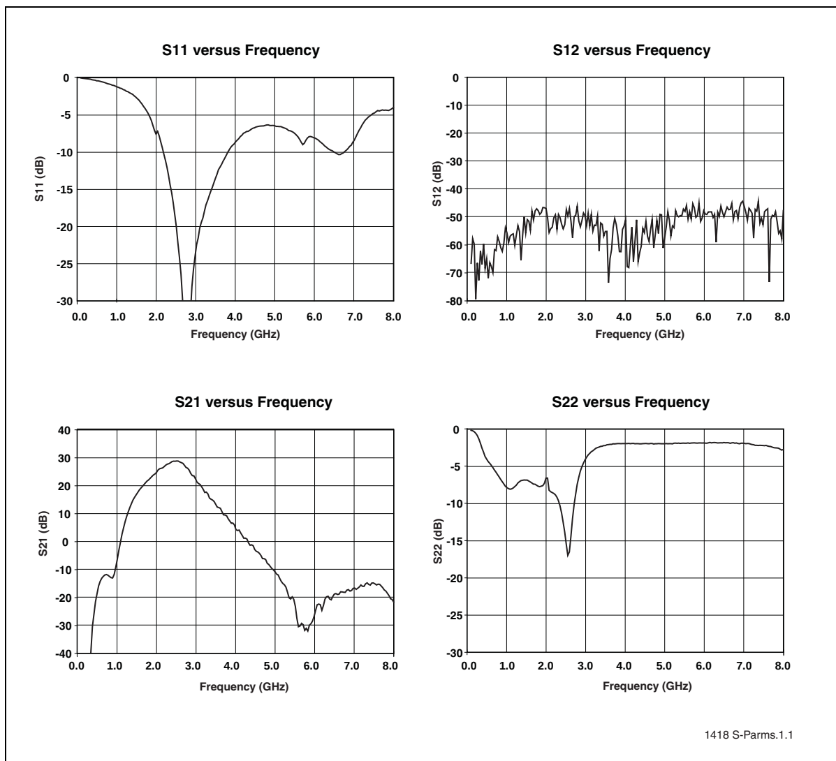
Figure 3: S-Parameters for TX Chain
