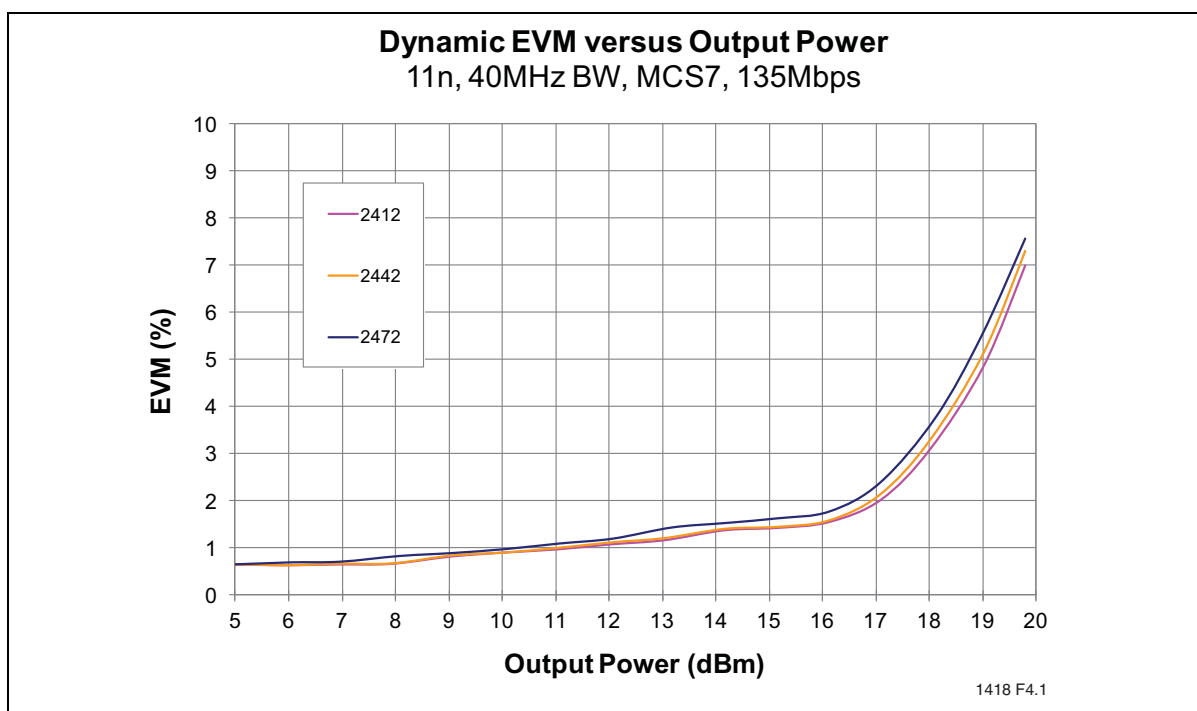
Figure 5: Dynamic EVM vs Output Power for MCS7-HT40 Modulation
