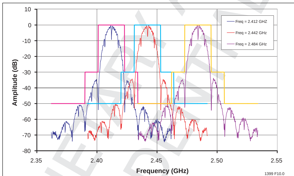
Figure 11: 802.11b Spectrum Mask at 23.5 dBm, Total Current 200mA
