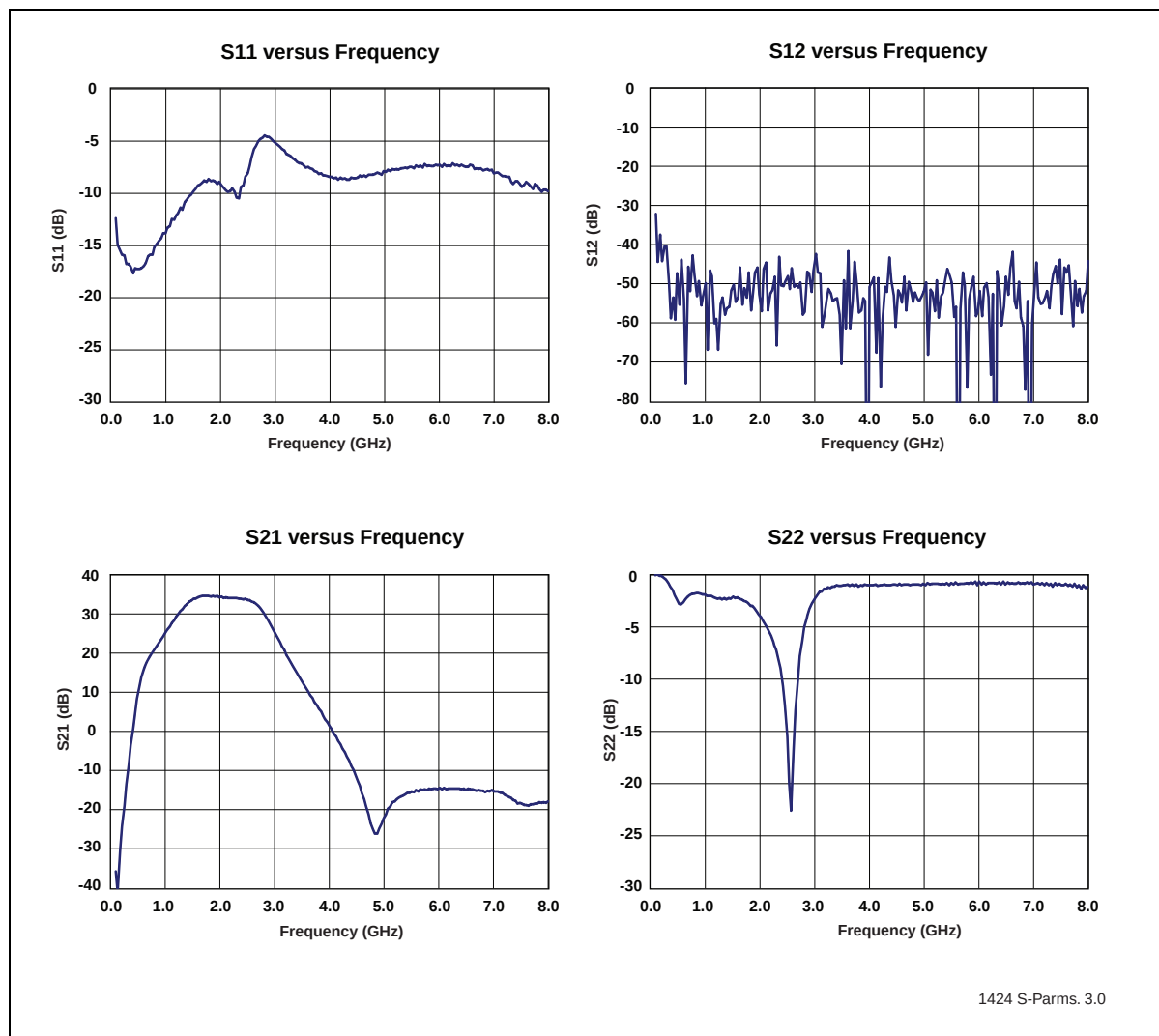
Figure 5: S-Parameters
