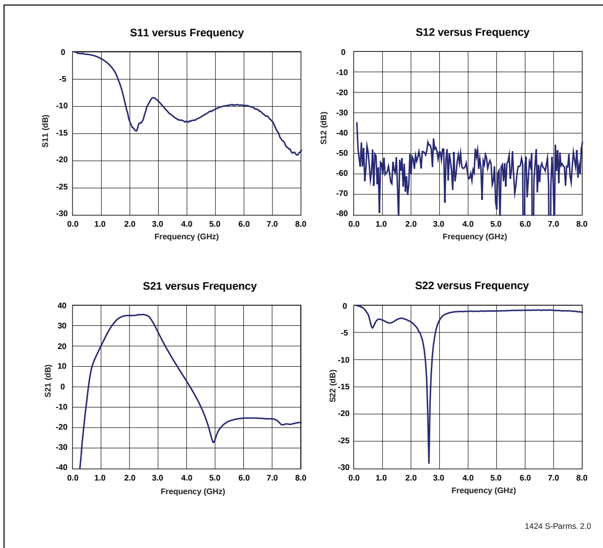
Figure 13: S-Parameters
