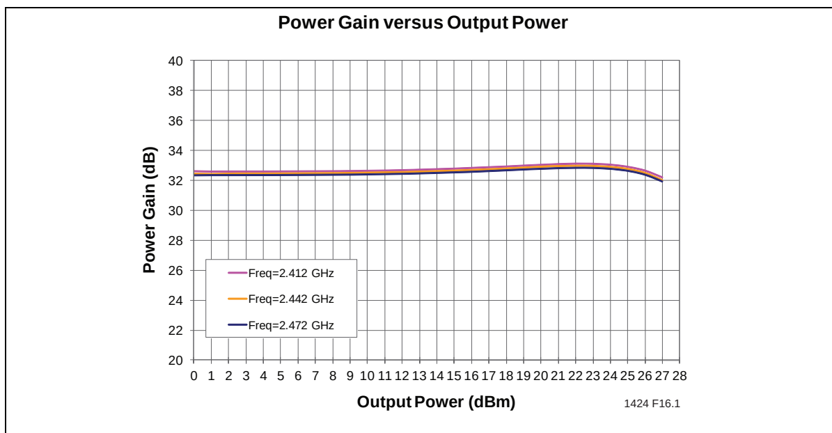
Figure 22: Gain versus Output Power
