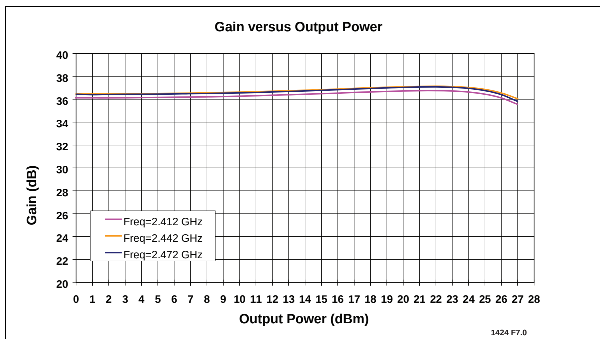
Figure 15: Gain versus Output Power
