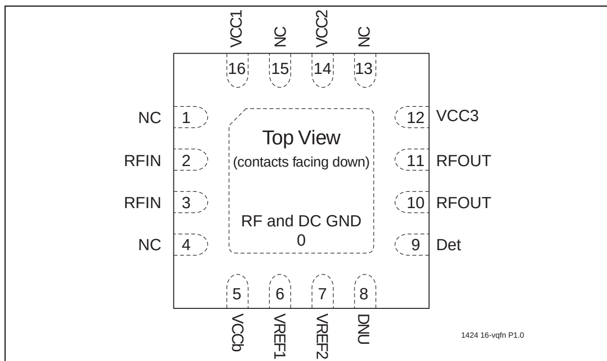
Figure 3: Pin Assignments for 3mm x 3mm, 16-contact VQFN (QVC)
