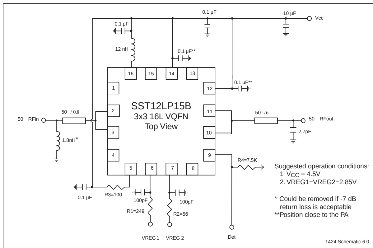
Figure 19: Typical Schematic for 4.5V, High-Efficiency 802.11b/g/n Applications for 16-contact VQFN
