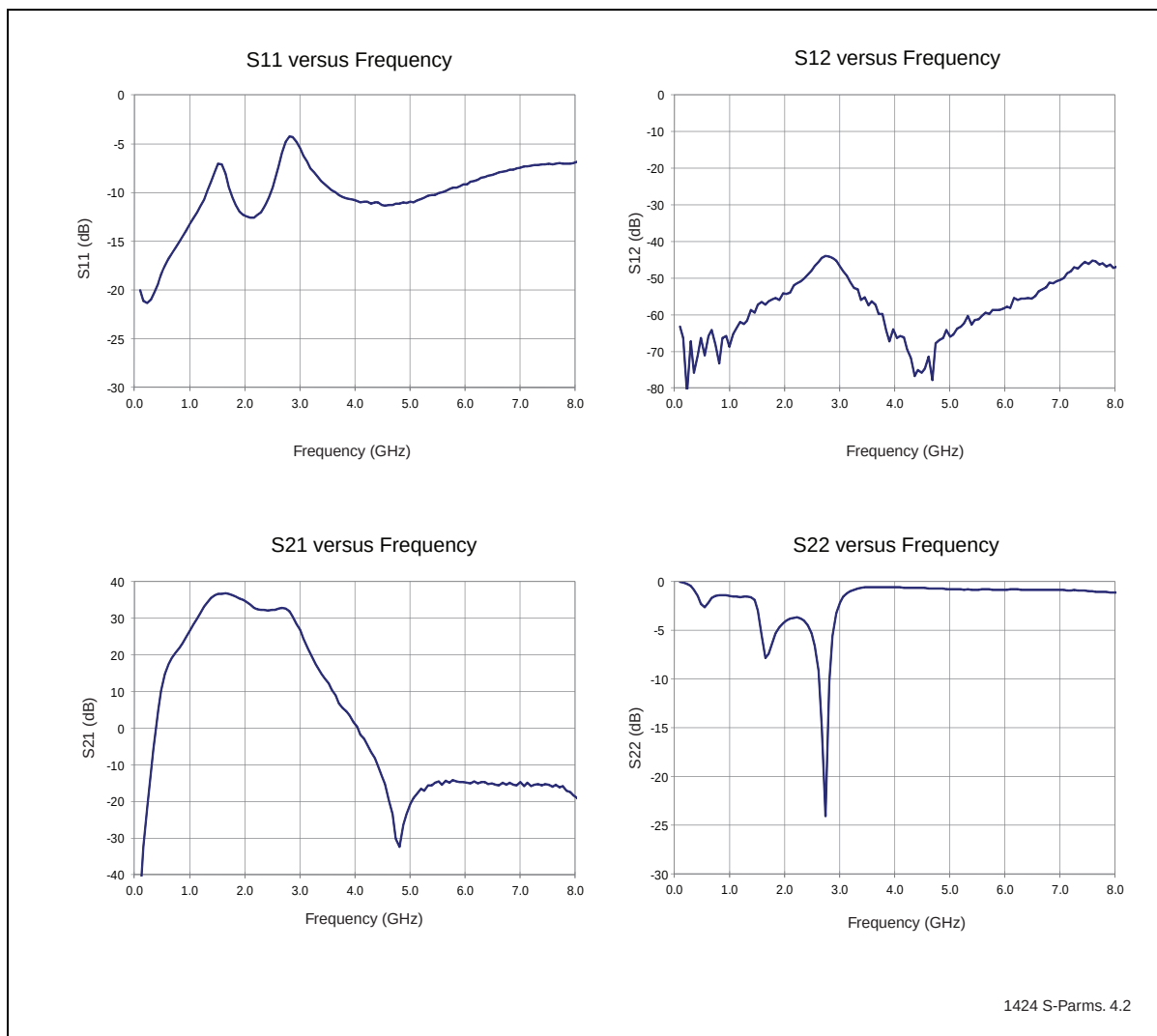
Figure 20: S-Parameters
