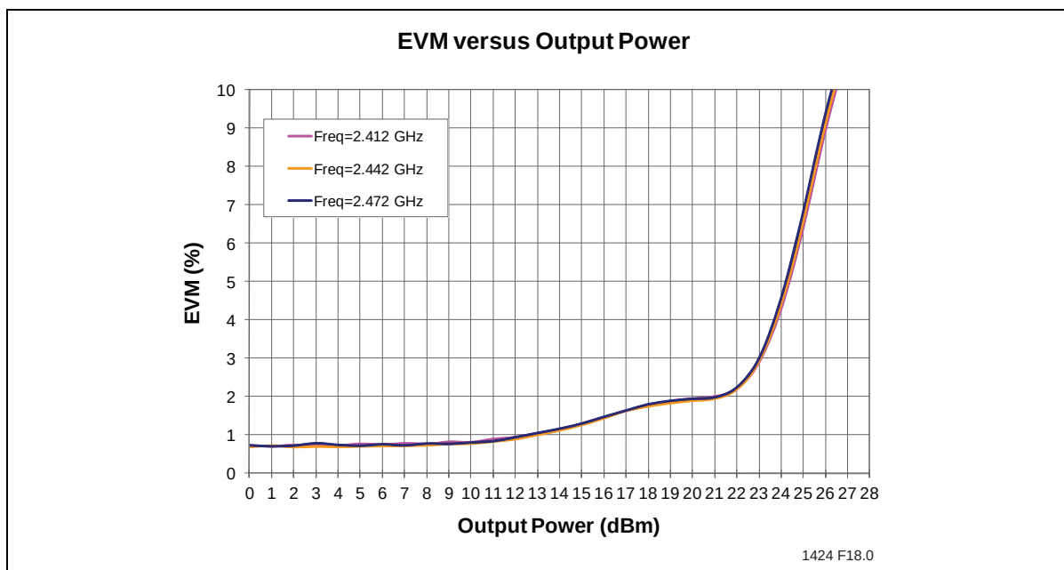
Figure 21: EVM versus Output Power measured with equalizer training set to sequence only
