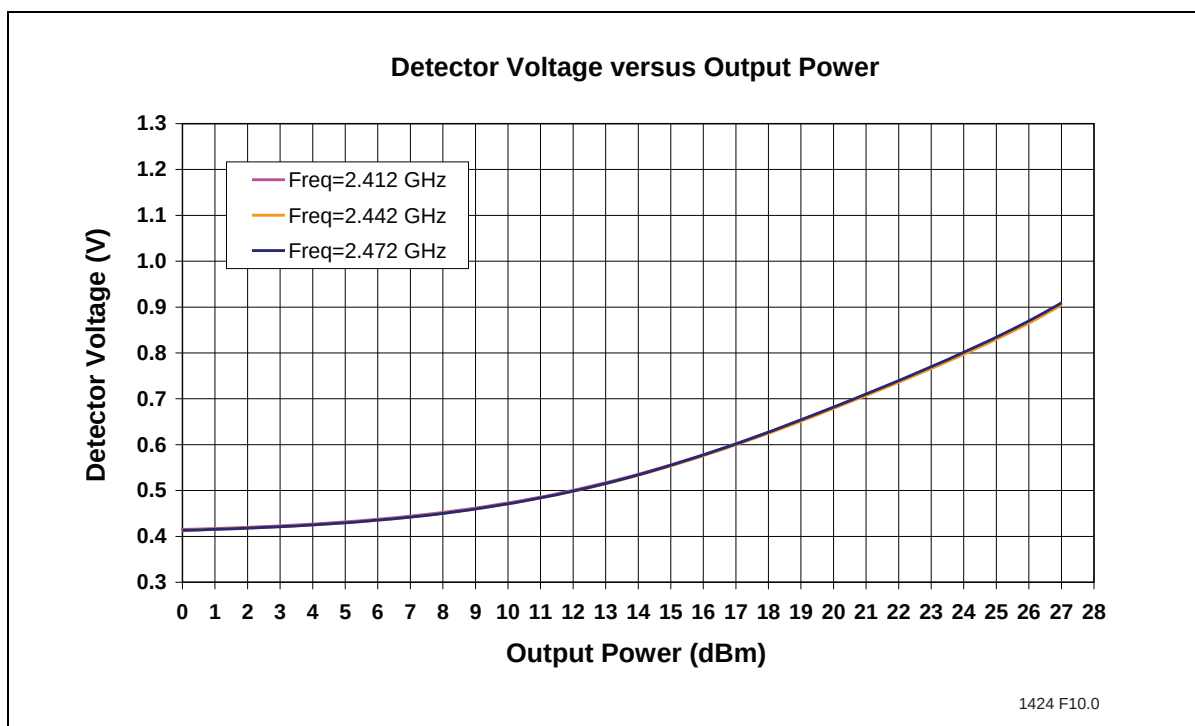
Figure 17: Detector Characteristics versus Output Power
