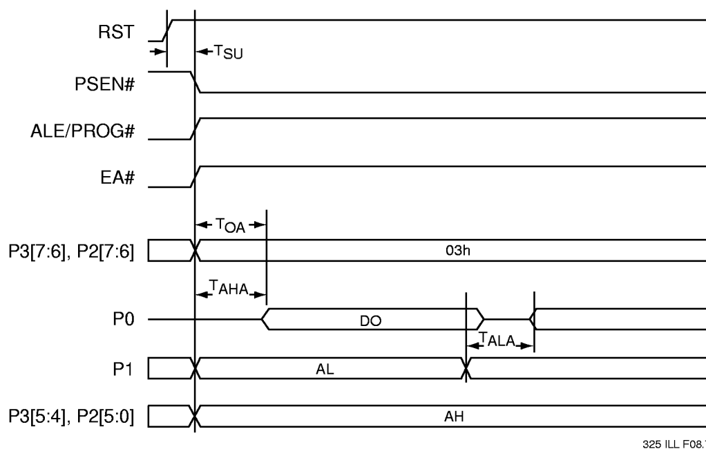
FIGURE 18: VERIFY BYTE
