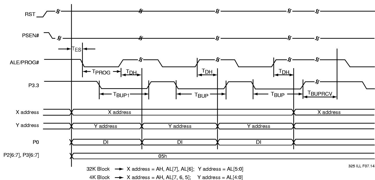
FIGURE 17: BURST PROGRAM
