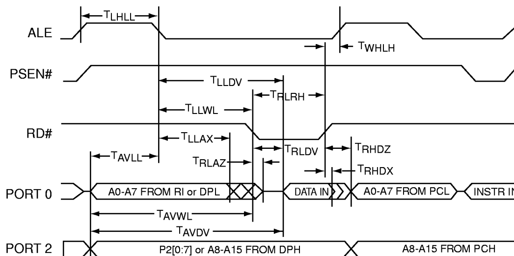
FIGURE 30: EXTERNAL DATA MEMORY READ CYCLE
