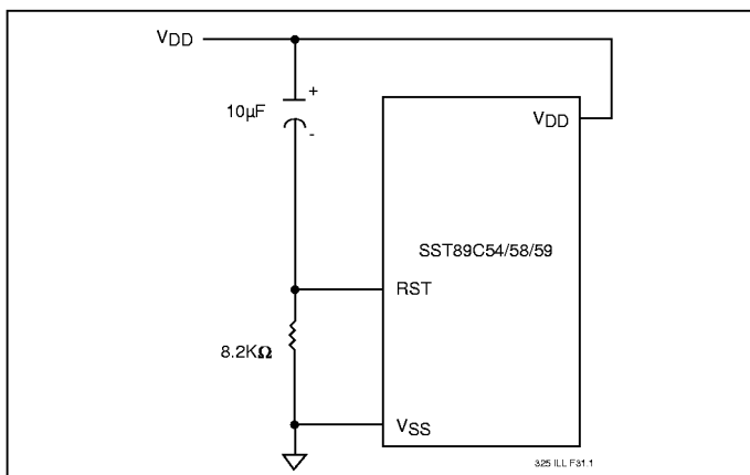
FIGURE 21: POWER-ON RESET CIRCUIT
