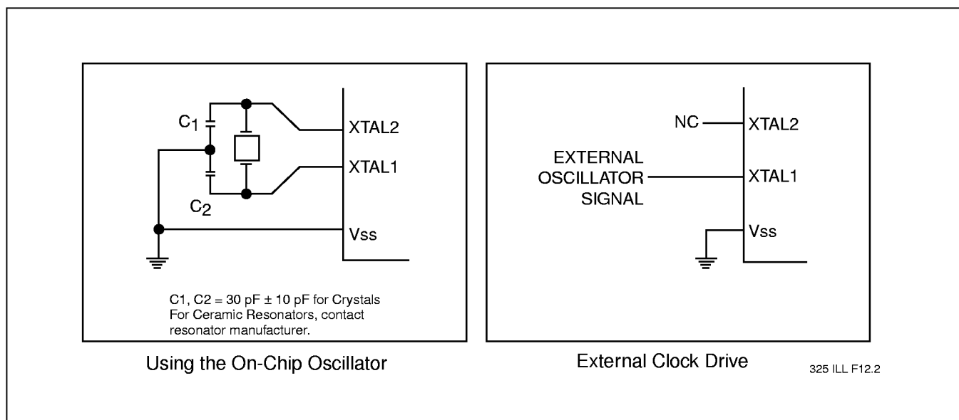
FIGURE 23: OSCILLATOR CHARACTERISTICS
