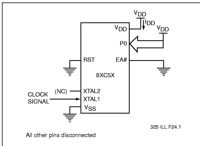
FIGURE 25: I_{DD} TEST CONDITION, IDLE MODE
