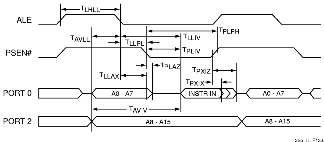
FIGURE 29: EXTERNAL PROGRAM MEMORY READ CYCLE
