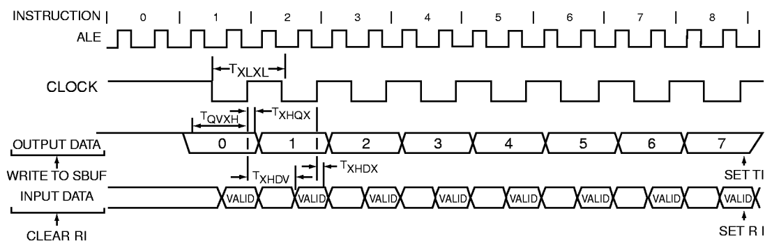
FIGURE 33: SHIFT REGISTER MODE TIMING WAVEFORMS
