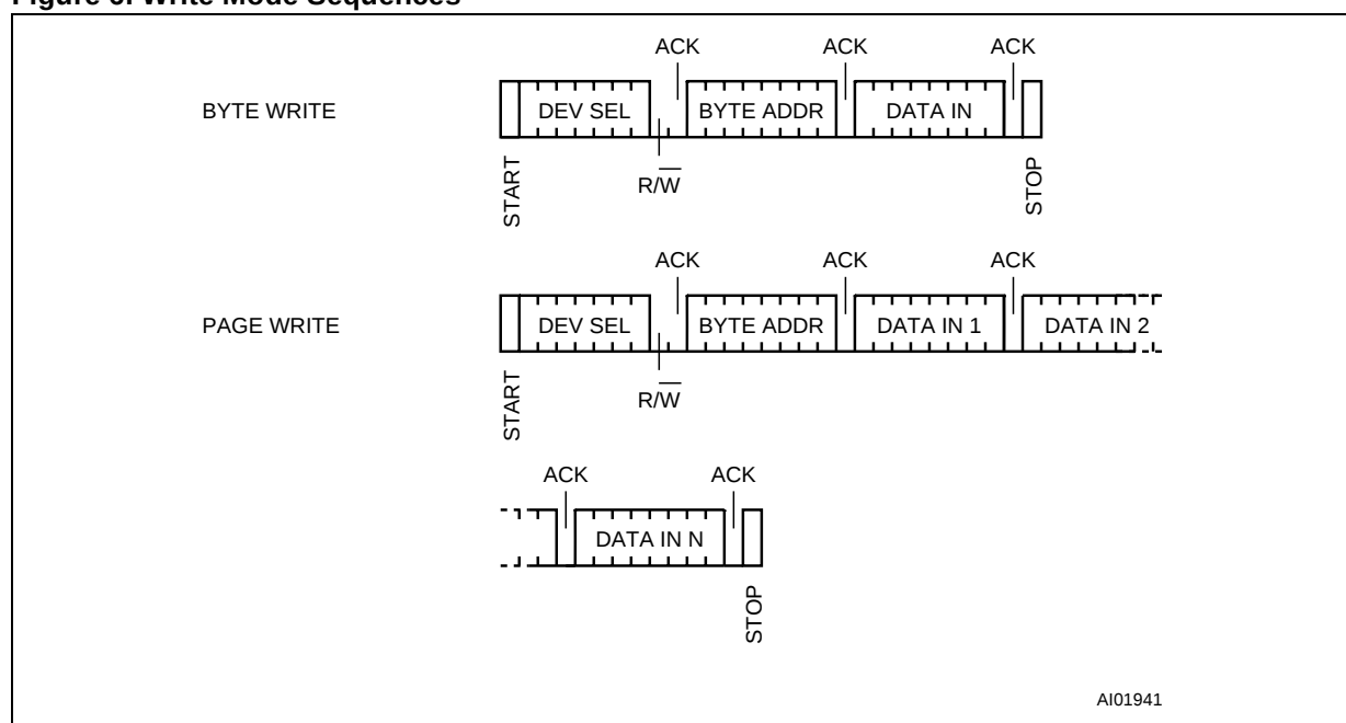
Figure 6. Write Mode Sequences
