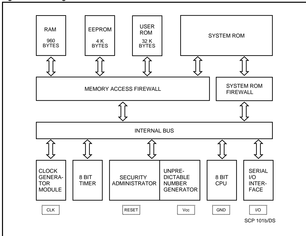
Figure 1. Block Diagram
