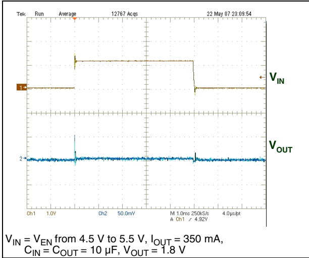
Figure 22. Line transient
