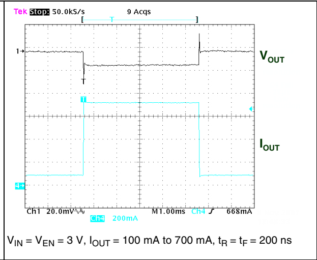
Figure 23. Load transient
