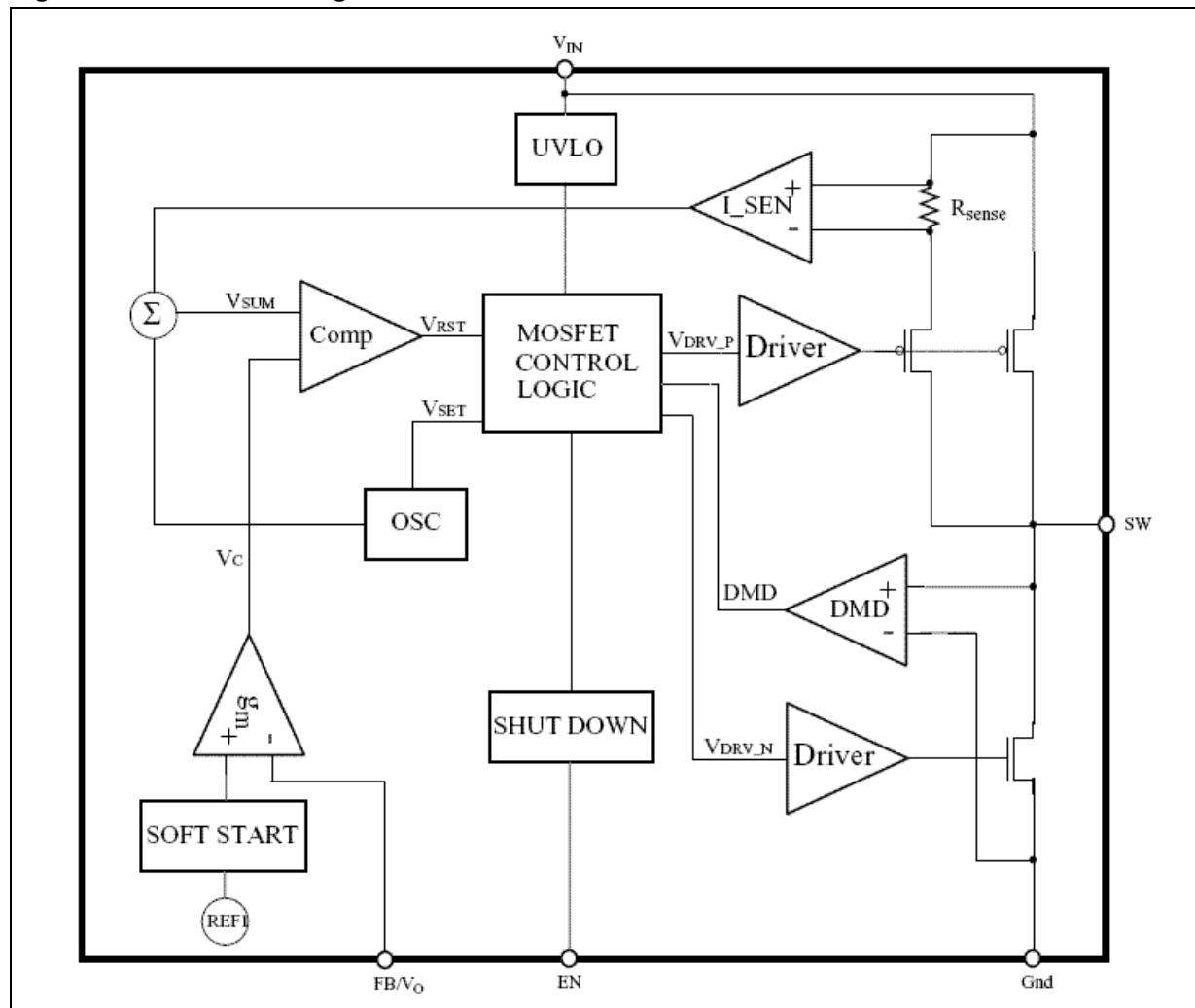
Figure 1. Schematic diagram
