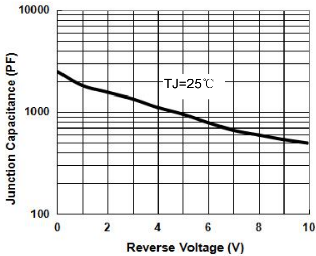
Fig.1-Typical Junction Capacitance
