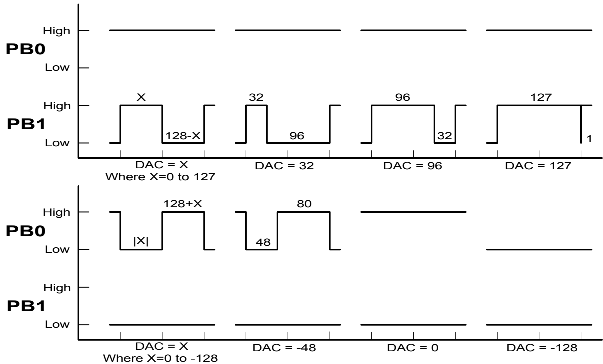
FIGURE 13-17: Two-Pin Two Ended PWM DAC Wave-form
