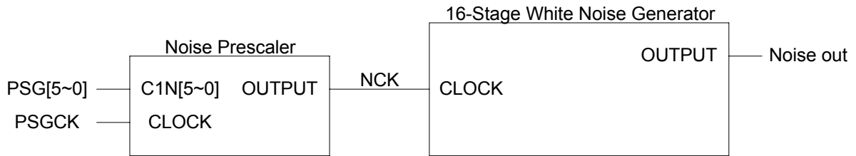
FIGURE 12-12: Noise Generator Diagram
