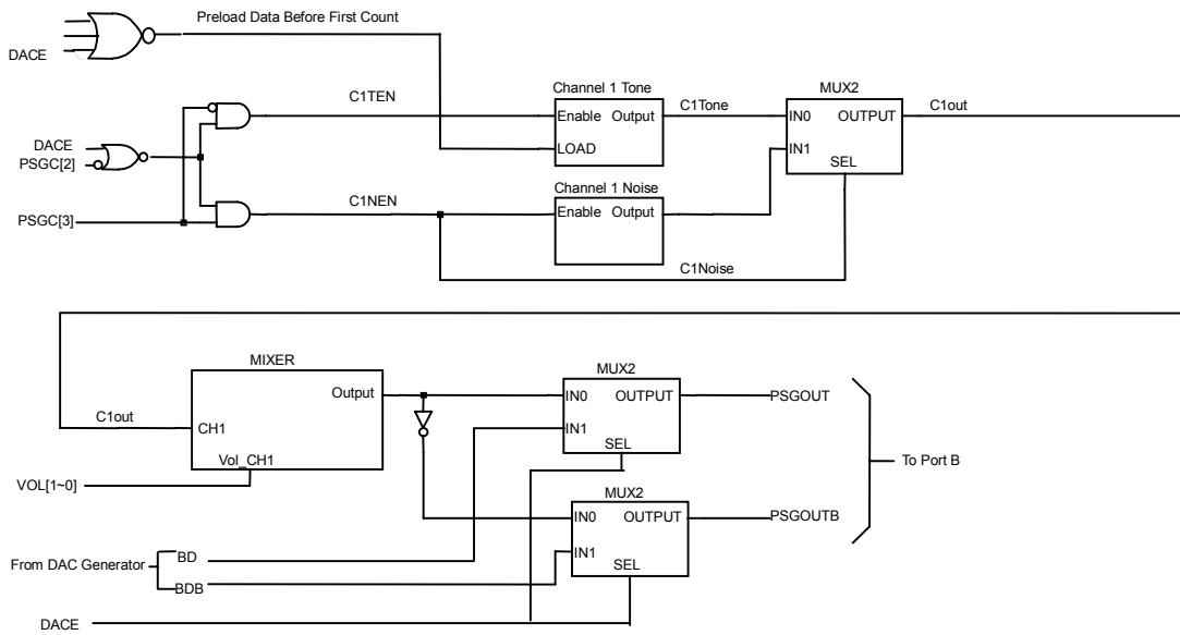
FIGURE 12-10: Program Sound Generator
