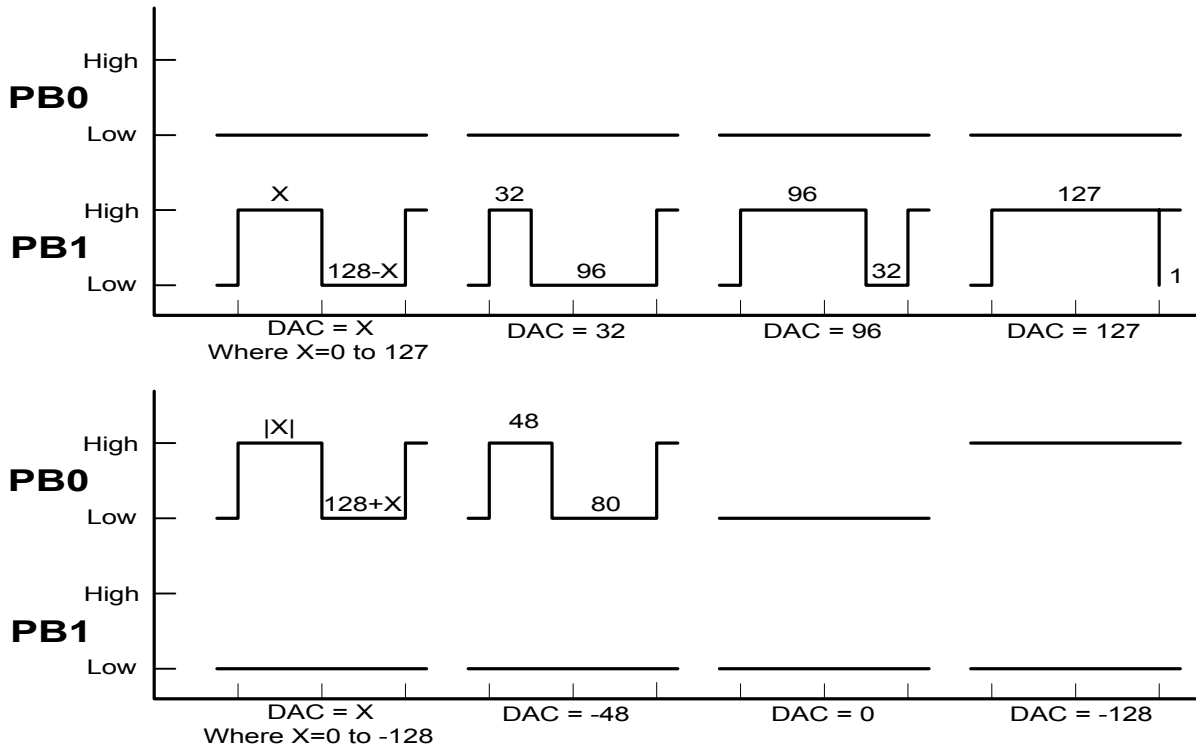
FIGURE 13-19: Two-Pin Push Pull PWM DAC Wave-form
