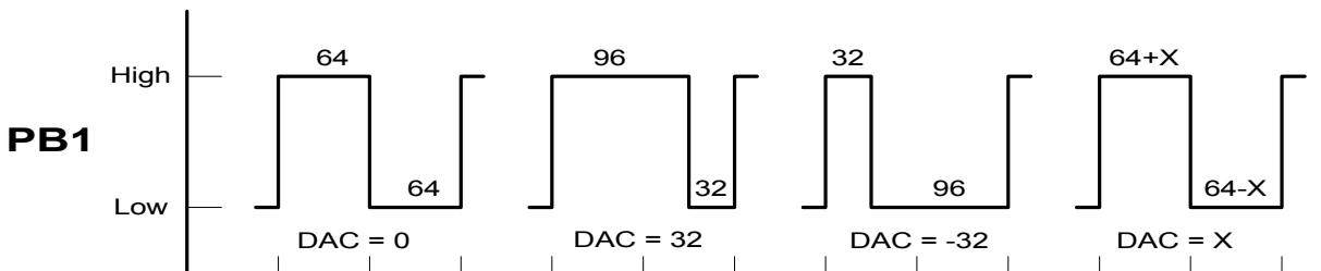
FIGURE 13-15: Single-Pin PWM DAC Wave-form
