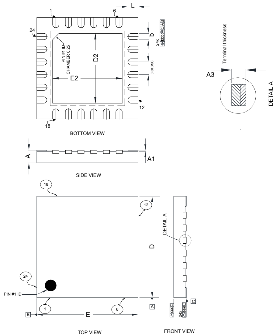
Figure 22. UFQFPN24 - Outline
