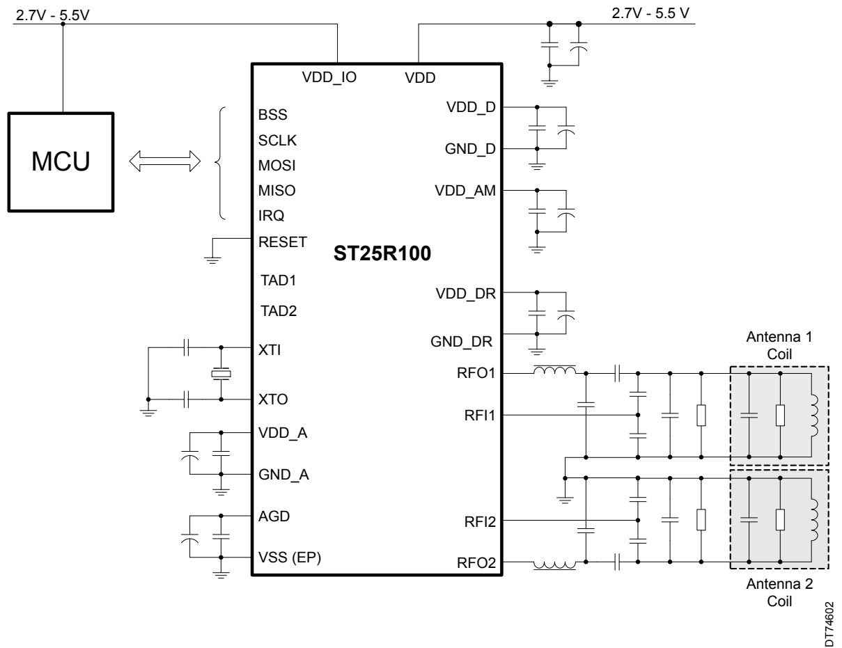
Figure 5. System diagram – two single-ended antenna driving
