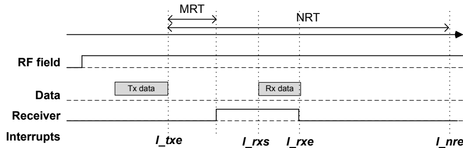
Figure 19. Transceiver operation with nrt_emd=1
