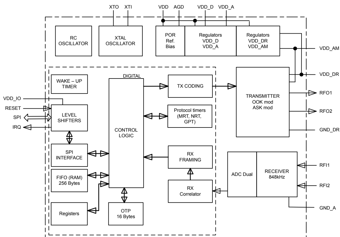
Figure 1. Block diagram
