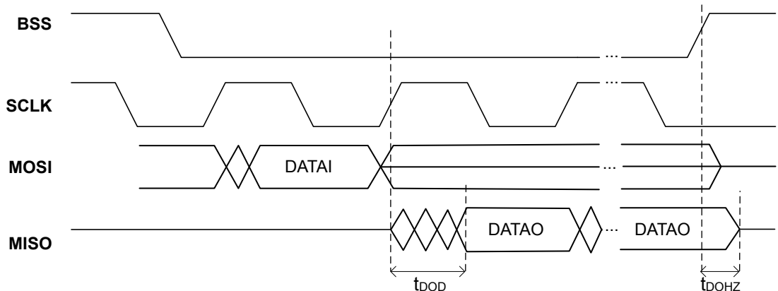
Figure 21. SPI timing diagram - Read operation
