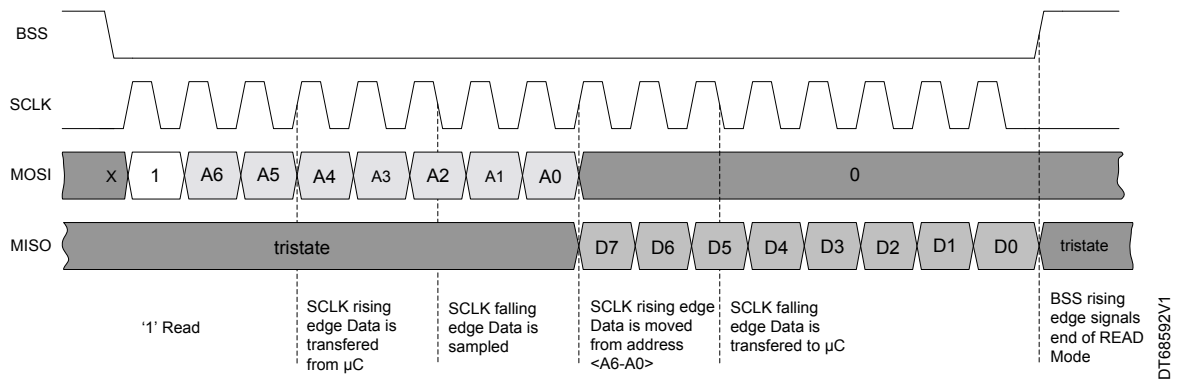
Figure 11. SPI communication: reading of single byte
