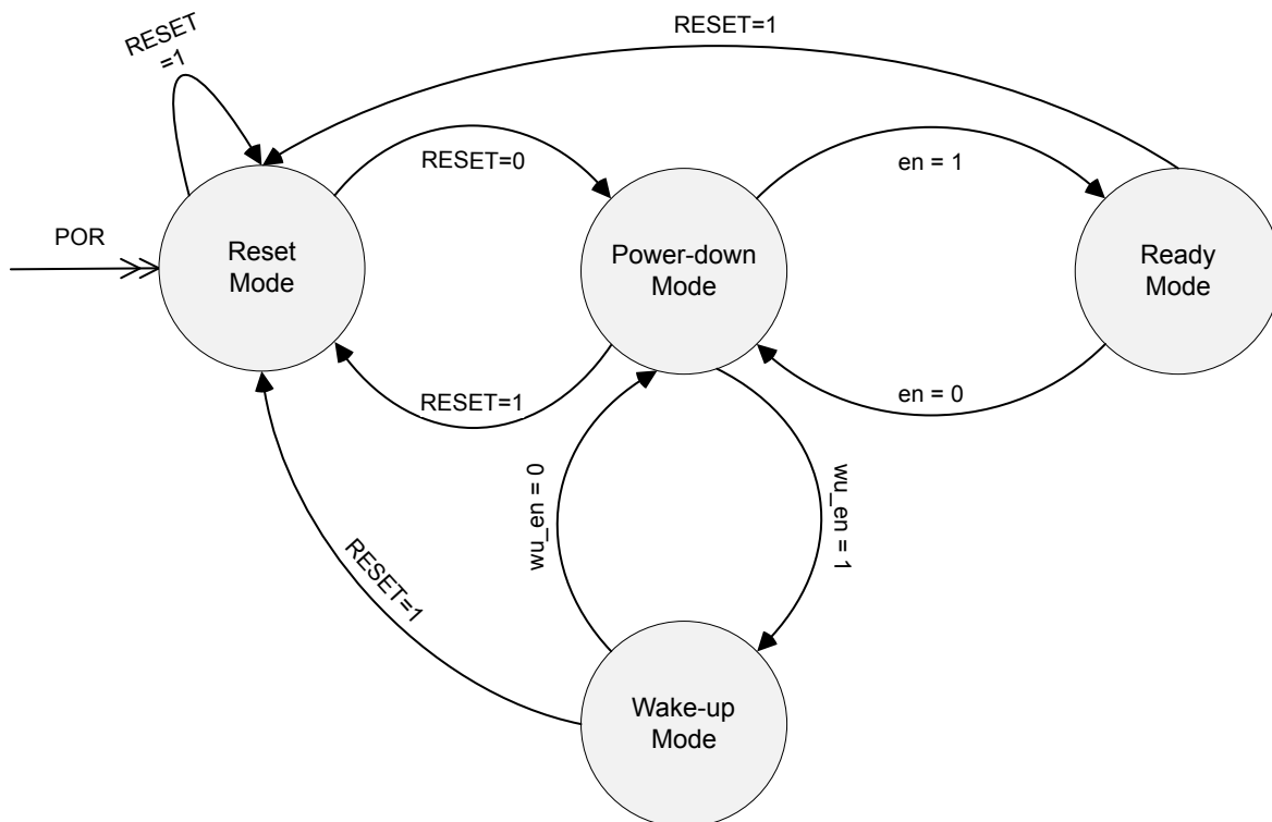
Figure 6. State diagram
