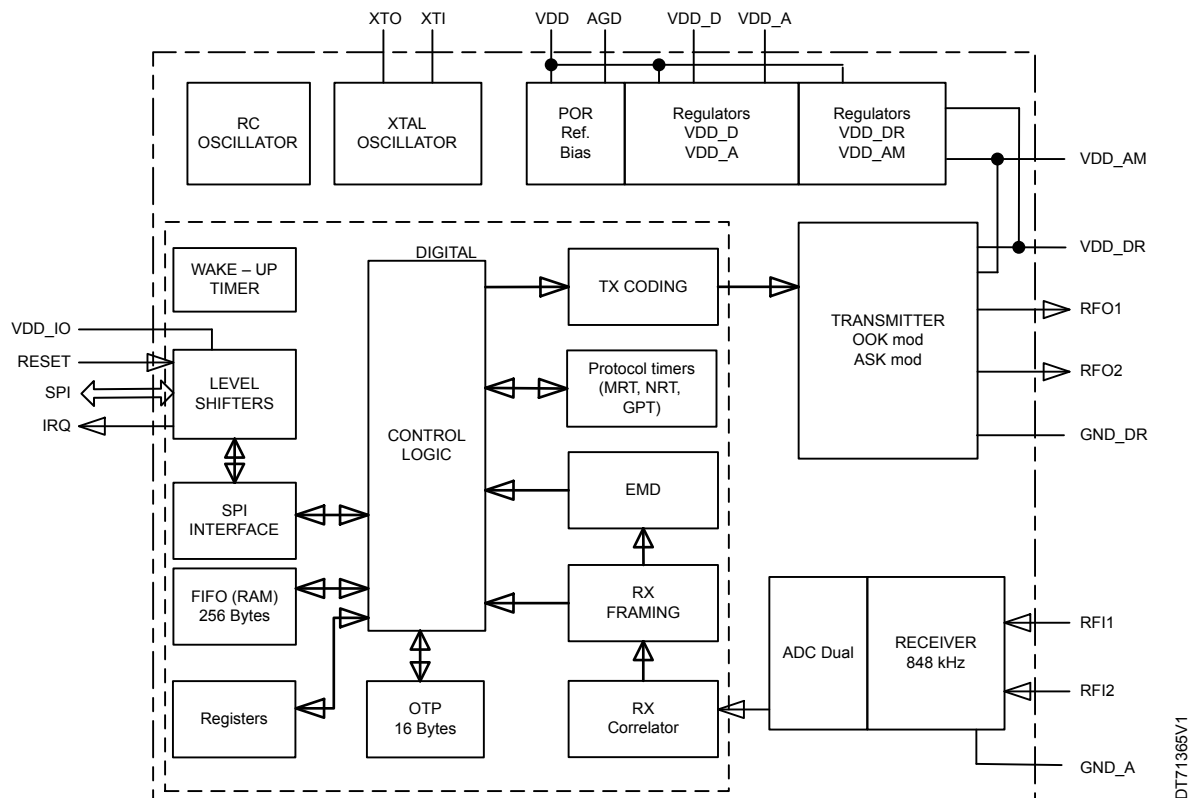
Figure 1. Block diagram
