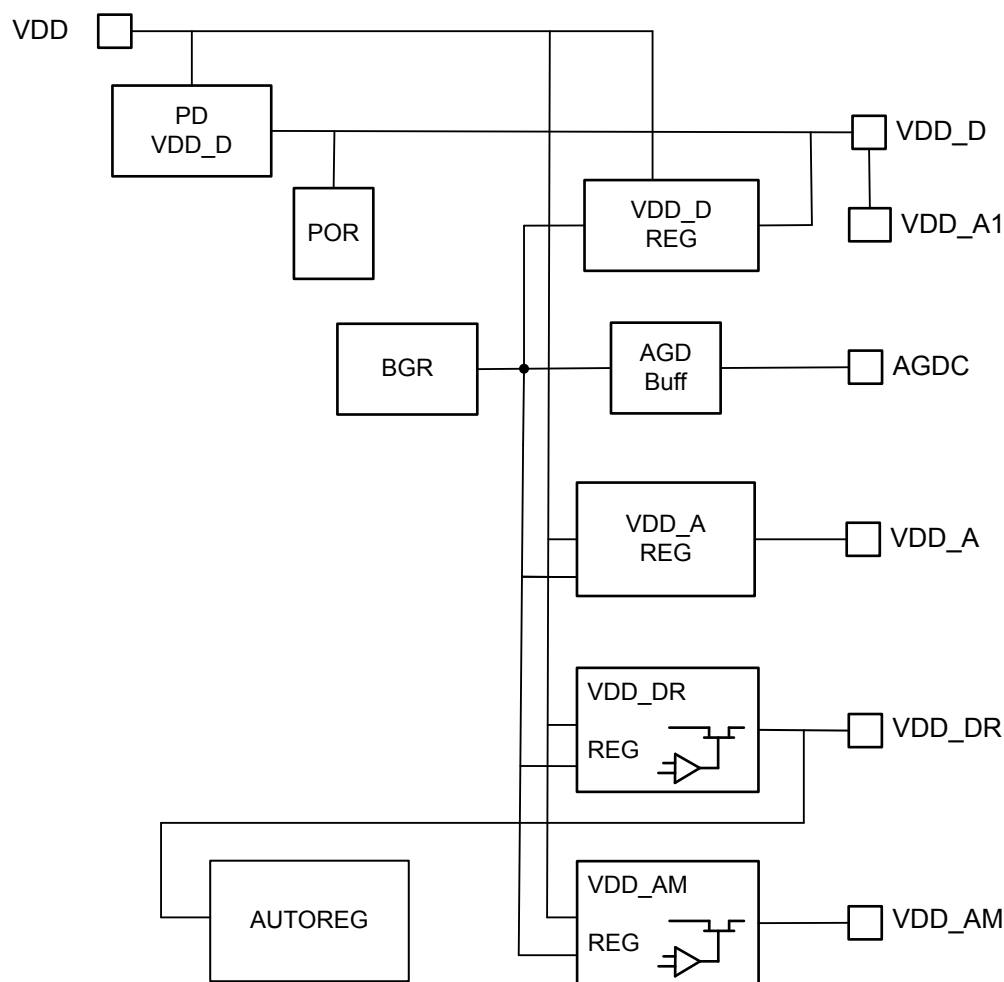
Figure 7. Supply system
