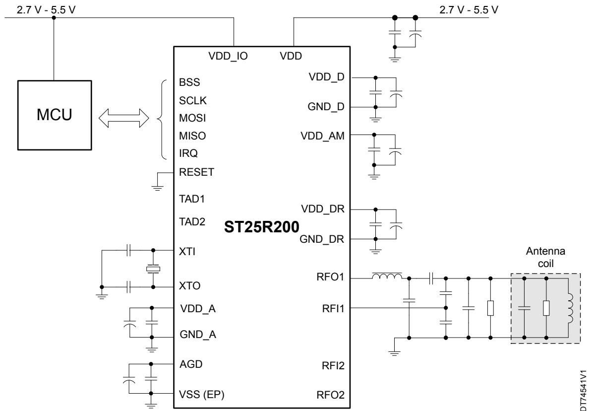
Figure 4. System diagram - single-ended antenna driving
