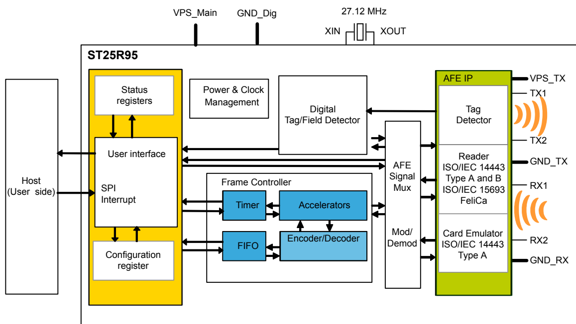
Figure 2. ST25R95 block diagram
